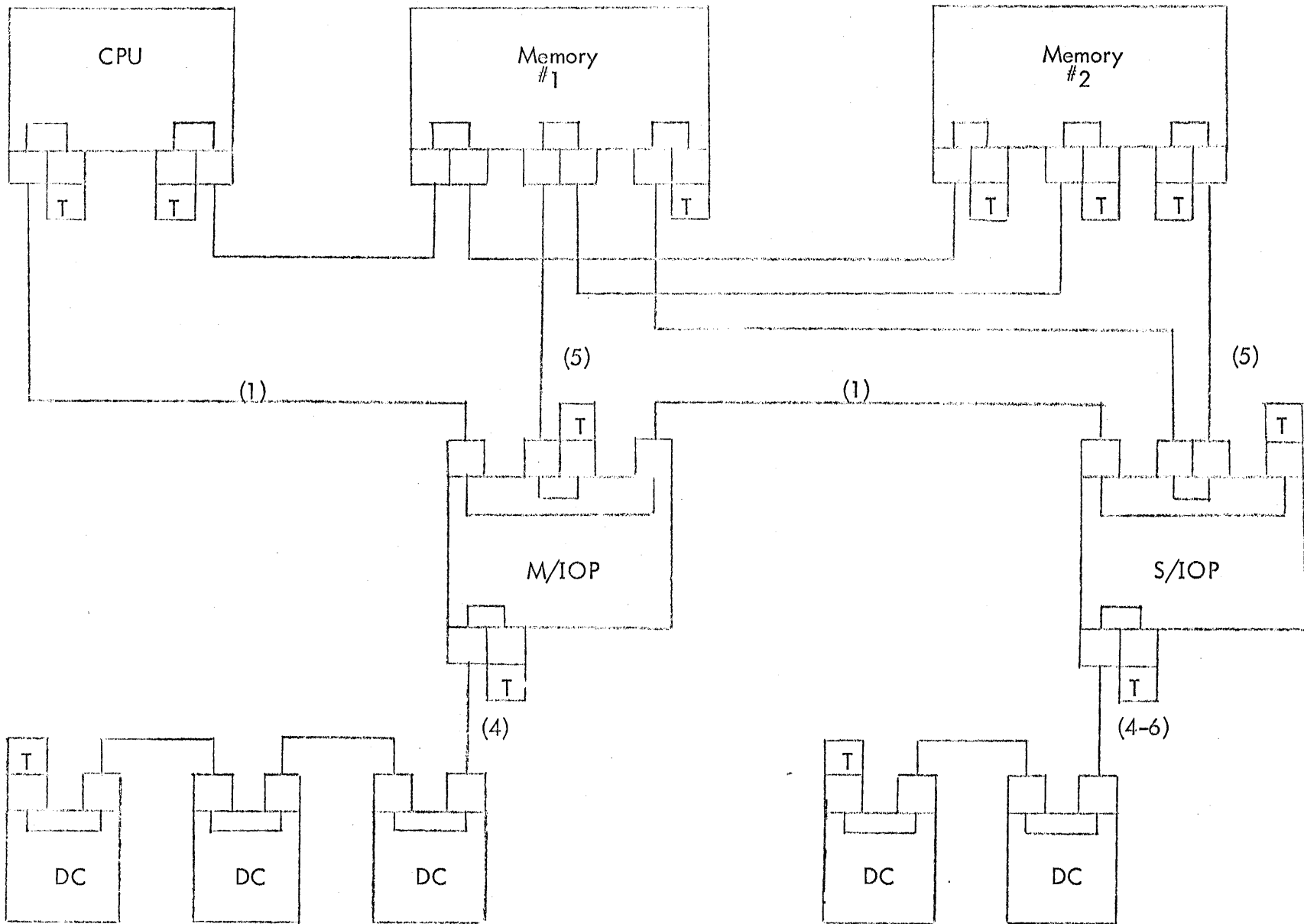
Figure 3.1 SYSTEM INTERCONNECTION
