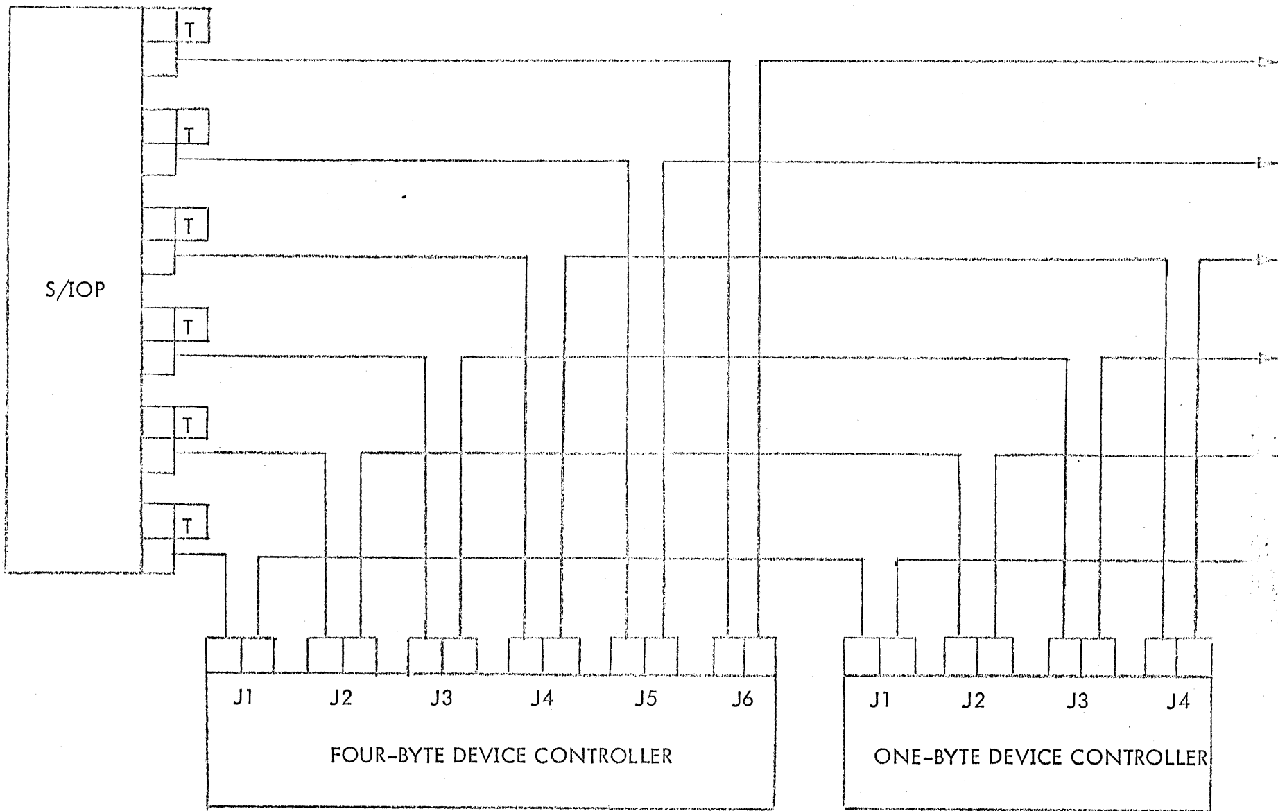
Figure 3.2 INTERCONNECTION OF S/IOP TO DEVICE CONTROLLERS
